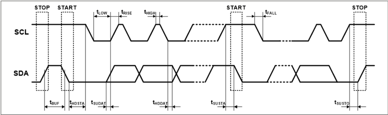
Figure 9: Serial interface timing diagram (串行接口时序图)
