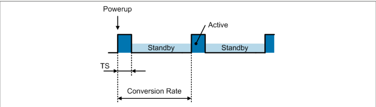
Figure 6: Conversion sequence ( 转换时序 )
