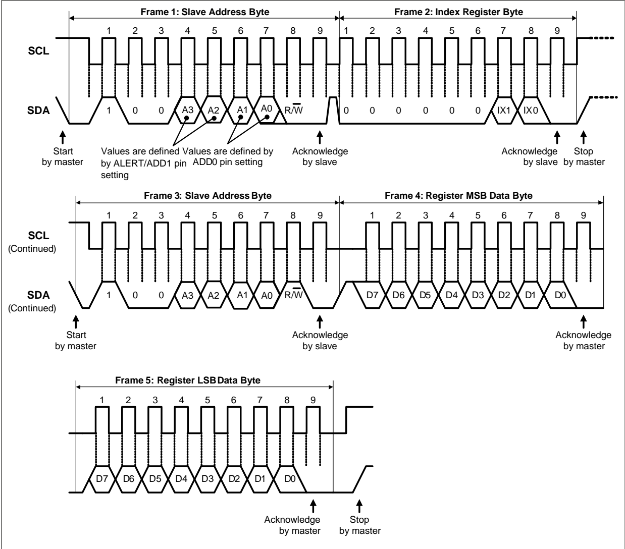
Figure 11: Timing diagram for word read ( 读字节时序图 )
