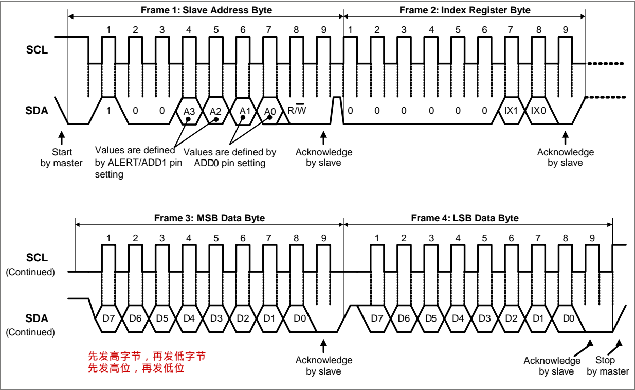
Figure 10: Timing diagram for word write ( 写字节时序图 )
